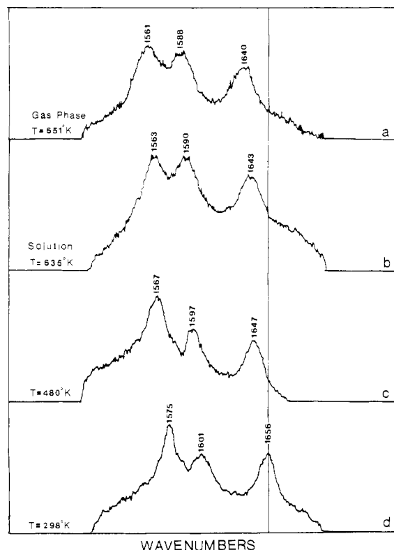
Figure 9. Resonance Raman spectra of nickel(II) octaethylporphine at band-pass \approx 4 \text{cm}^{-1} : (a) in the gas phase, T = 651 K, \lambda_{\text{ex}} = 5543 Å, laser power = 0.25 W; (b-d) in diffusion oil at the temperature indicated in the figure, \lambda_{\text{ex}} = 5544 Å, laser power = 0.03 W for b and 0.1 W for c and d. The contribution of diffusion oil to the Raman spectra was subtracted out of spectra b, c, and d by numerically subtracting diffusion-oil spectra obtained at each of the individual temperatures.
