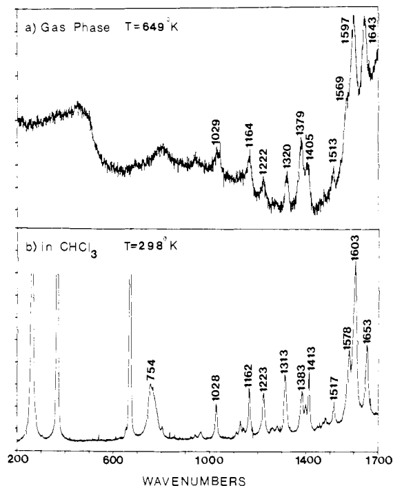
Figure 8. Resonance Raman spectra of cobalt(II) octaethylporphine: (a) in the gas phase, T = 649 K, \lambda_{\text{ex}} = 5145 Å, laser power = 1.2 W, band-pass \approx 4 \text{cm}^{-1} , counting time = 1 s, scans = 2; (b) in \text{CHCl}_3 at room temperature, \lambda_{\text{ex}} = 5145 Å, laser power = 0.5 W, band-pass \approx 4 \text{cm}^{-1} , counting time = 1 s, scans = 1.
