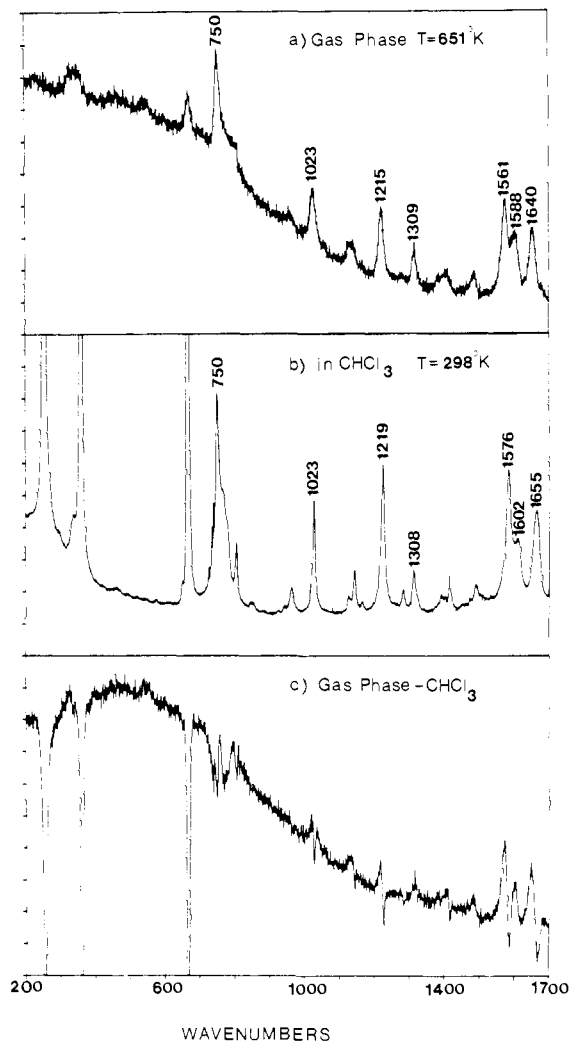
Figure 7. Resonance Raman spectra of nickel(II) octaethylporphyrine (a) in the gas phase, T = 651 K, \lambda_{ex} = 5565 Å, laser power = 0.5 W, band-pass \approx 4 cm -1 , counting time = 1 s, scans = 2; (b) in CHCl 3 solution at room temperature, \lambda_{ex} = 5564 Å, laser power = 0.2 W, band-pass \approx 4 cm -1 , counting time = 1 s, scans = 1; and (c) as a difference spectrum (spectrum a - spectrum b), peaks below 700 cm -1 in parts b and c which are off scale derive from the solvent CHCl 3 .
