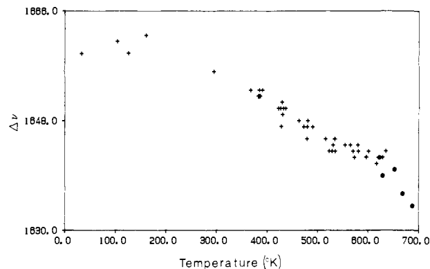
Figure 10. Temperature dependence of the \nu_{10} vibrational frequency of Nickel(II) octaethylporphine. The crosses label frequencies of \nu_{10} in diffusion-oil solutions of NiOEP, while the circles label the frequencies in the gas-phase samples.
